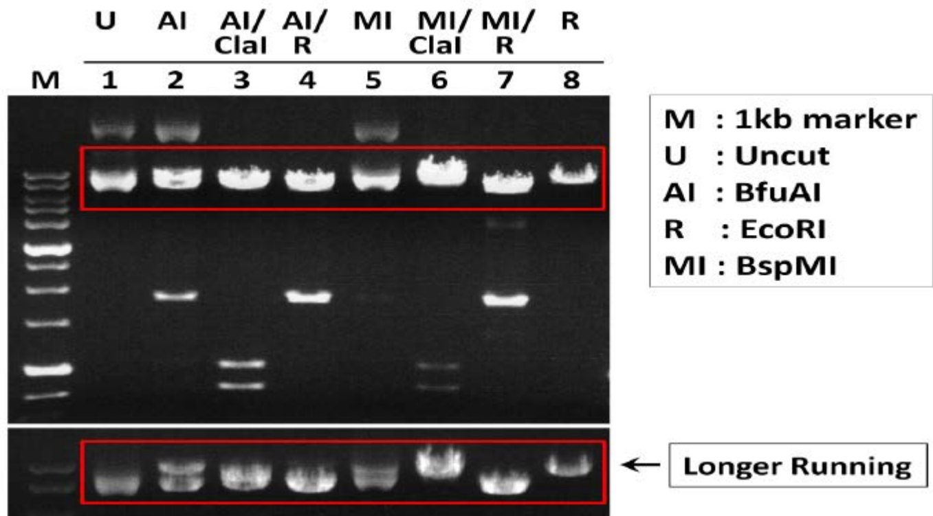
Figure 2A. A double digestion of BfuAI / BspMI plus EcoRI efficiently restricts the plasmid of pLAS1.3xLacO for shRNA cloning. Each lane contained 200 ng of pLAS1.3xLacO (Digestion was performed in a volume of 12ul with restriction enzymes less than 0.8ul). Although the 1.9 kb fragment of the plasmid is flanked by 2 BspMI and BfuAI cutting site, our results showed that a single RE digestion of BspMI or BfuAI could not completely remove the fragment (Lane 2 & 5). A double digestion of BspMI or BfuAI with Clal is not recommended due to different buffer requirement is needed to achieve optimal result (Lane 3 & 6). A double digestion of EcoRI and BfuAI is recommended for preparing this vector. The conditions are as follows: DNA first digests with EcoRI for appropriate time to ensure the plasmid DNA is linearized, then add BfuAI directly to EcoRI -digested mixture and incubate at 50°C for at least two hrs (Lane 4). A double digestion of BspMI and EcoRI could also achieve the same efficiency in fragment removal as its isoschizomer applied (Lane 7).
