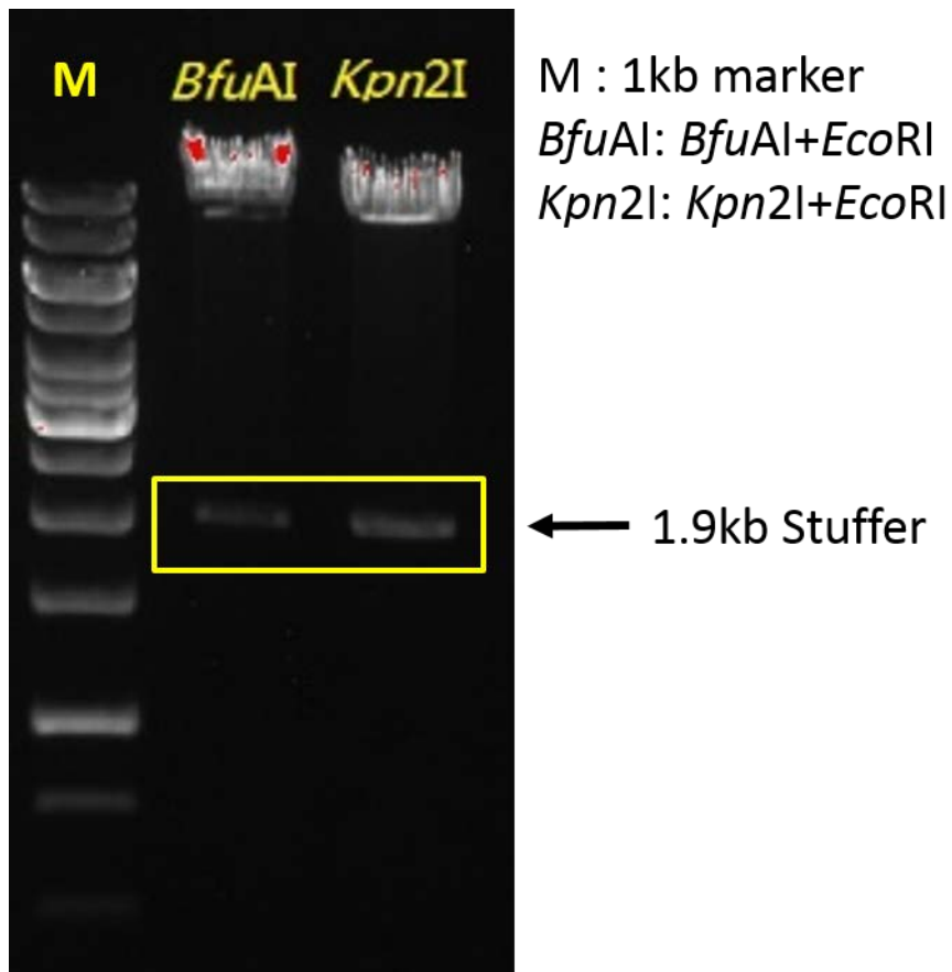
Figure 2B. The plasmid of pLAS1.3xLacO-M2 for shRNA cloning , which double digestion of Kpn2I plus EcoRI is more efficiency than BfuAI plus EcoRI .
