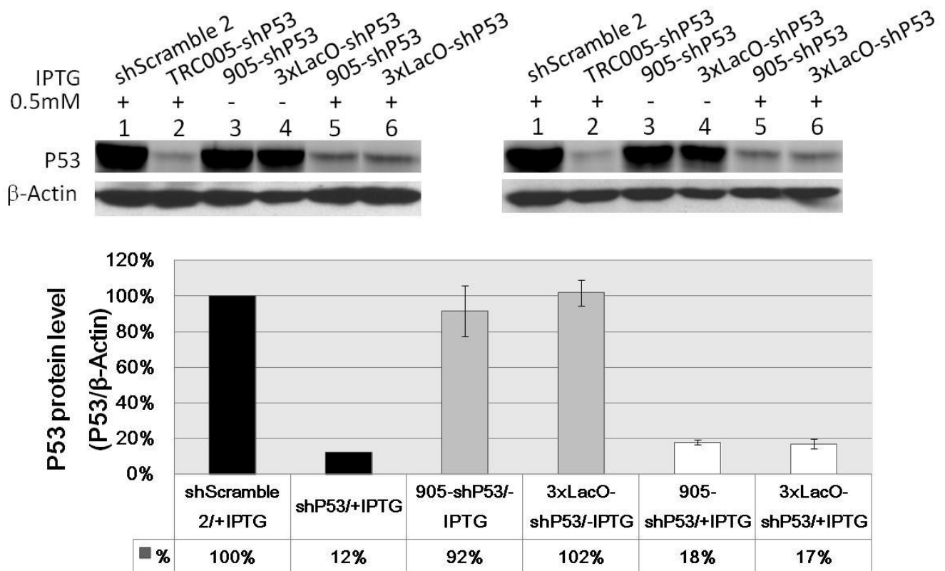
Figure 3. Tightness and responsibility of pLAS1.3xLacO vector . The results of lower panel were obtained from two independent experiments shown in upper panel. 905-shP53 was derived from TRC vector called pTRC-905, which also contains 3 copies of LacO operator but one of the LacO operator location is different from pLAS1.3xLacO. Western blotting lysate preparation . Cell was washed with cold PBS, scraped, then centrifuged to pellet the cell, supernatant was removed and appropriate volume of CellLysis M reagent (Sigma #C2978) supplemented with protease inhibitor cocktail (Roche #04693132001) was added, Incubate at RT for 30 mins then centrifuge for 15 mins, 13000 rpm. Next, lysate was transferred into pre-cooled 1.5 ml microcentrifuge tube for further western analysis.
