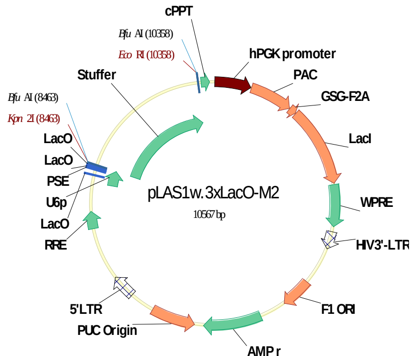
Figure 1. Map of pLAS1w.3xLacO-M2 . pLAS1w.3xLacO-M2 was derived from pLKO_TRC005 with the following modifications:
